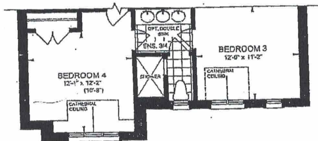
PARTIAL SECOND FLOOR PLAN ELEVATION B
