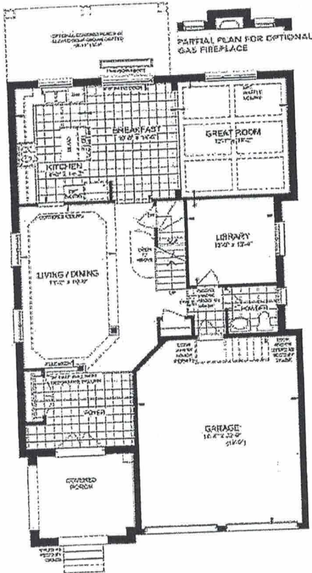
GROUND FLOOR PLAN ELEVATION A
