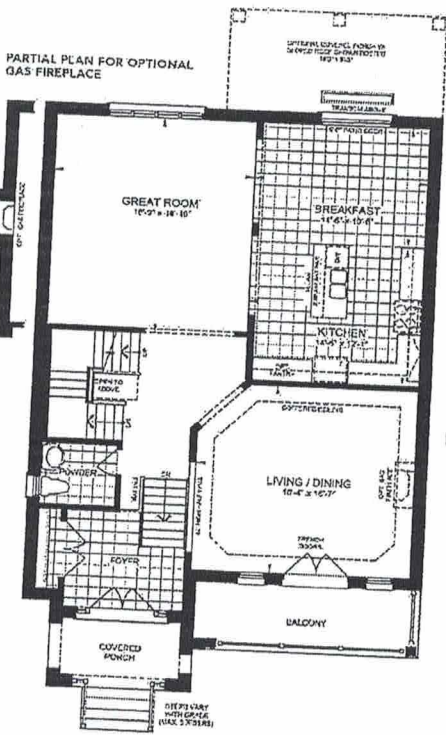
GROUND FLOOR PLAN ELEVATION A
