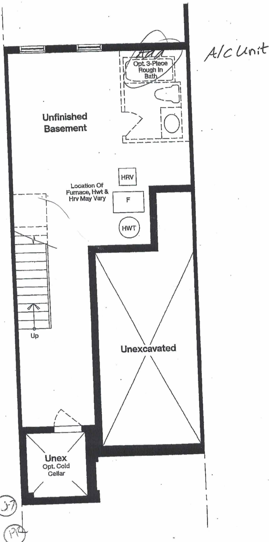
BASEMENT PLAN
