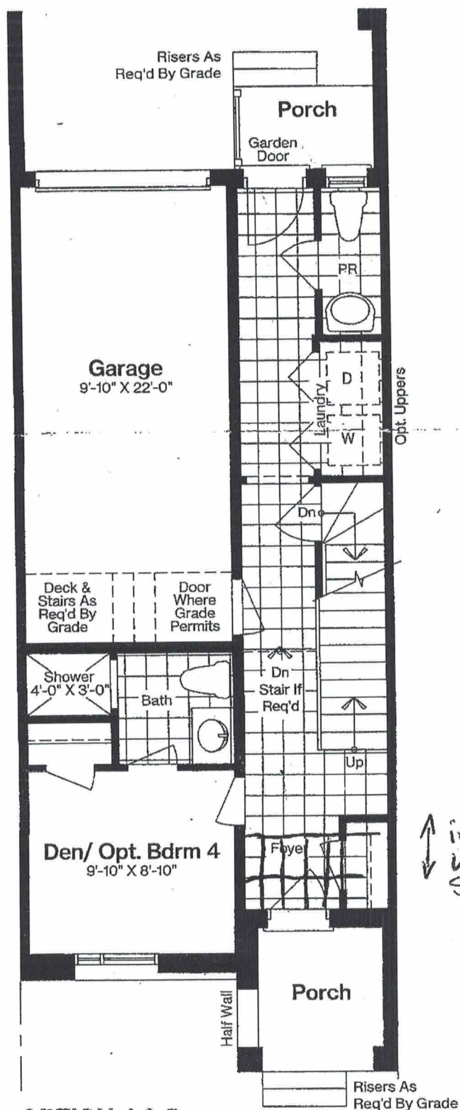
OPTION 4 & 5: ALTERNATE DEN/4 BEDROOM LAYOUT FIRST FLOOR PLAN
