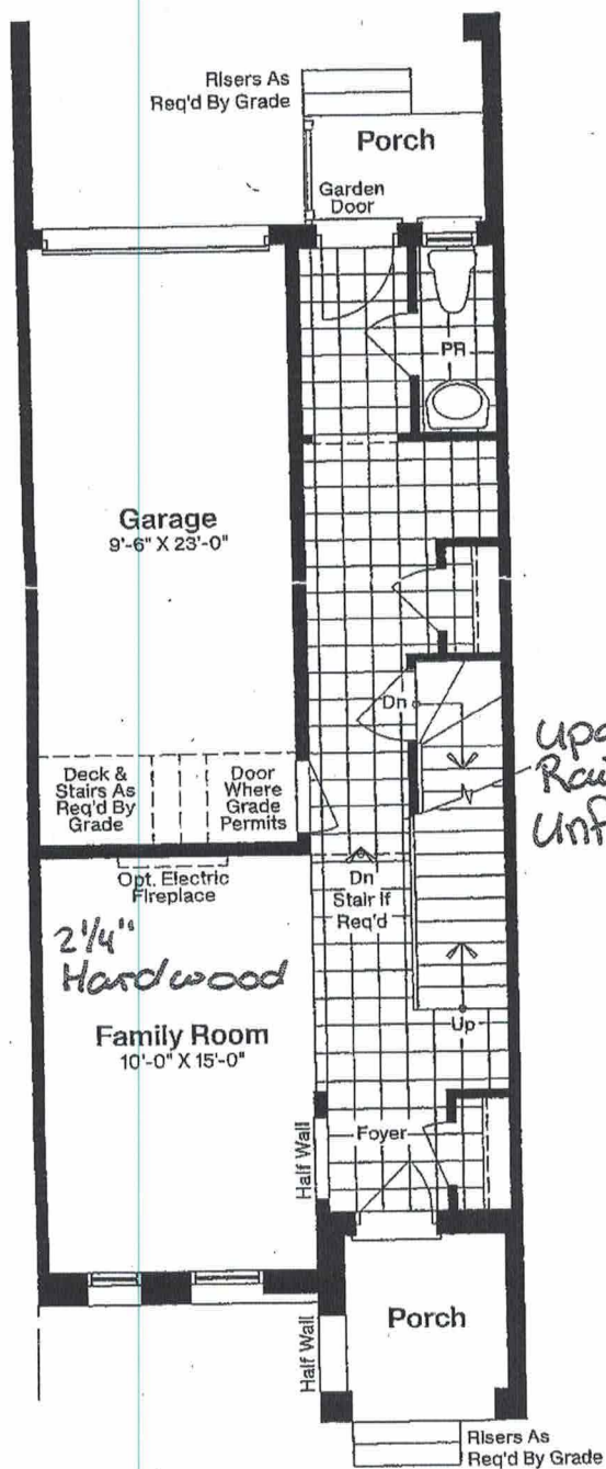
OPTION 3: OPTIONAL SECOND FLOOR LAUNDRY LAYOUT FIRST FLOOR PLAN
