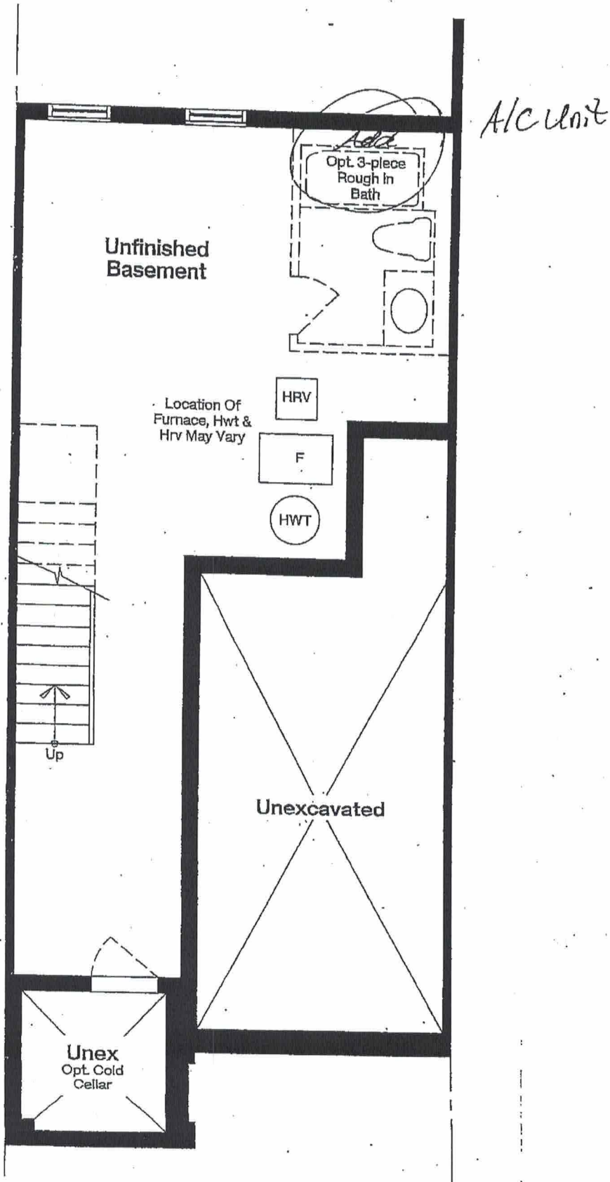
BASEMENT PLAN
