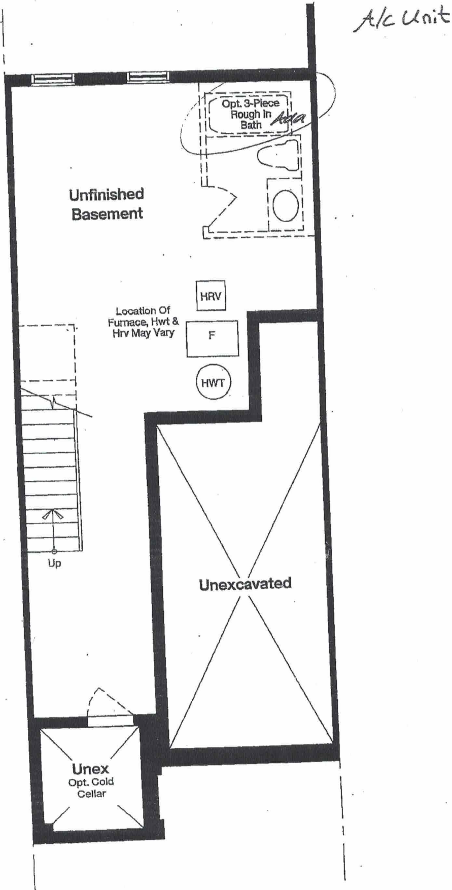
BASEMENT PLAN
