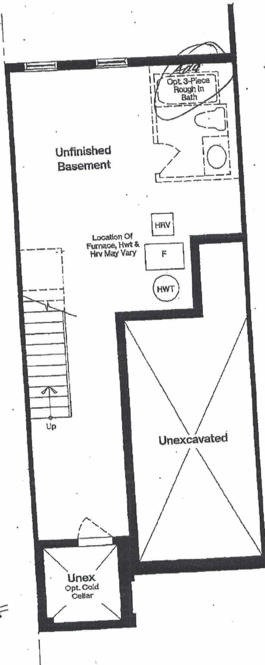
BASEMENT PLAN
