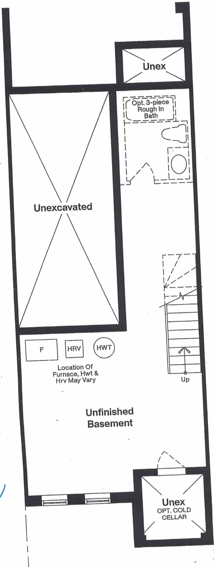
BASEMENT PLAN
