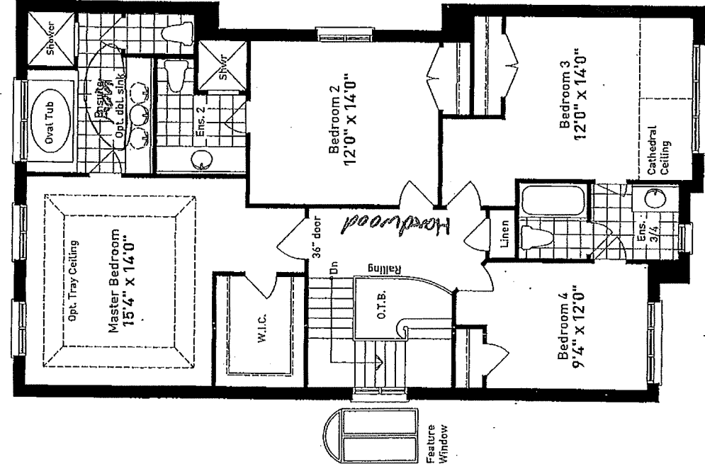
SECOND FLOOR PLAN ELEVATION B
