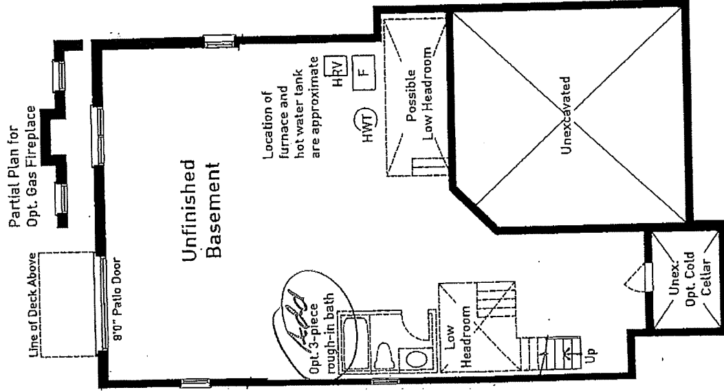
WALKOUT BASEMENT FLOOR PLAN ELEVATION A
