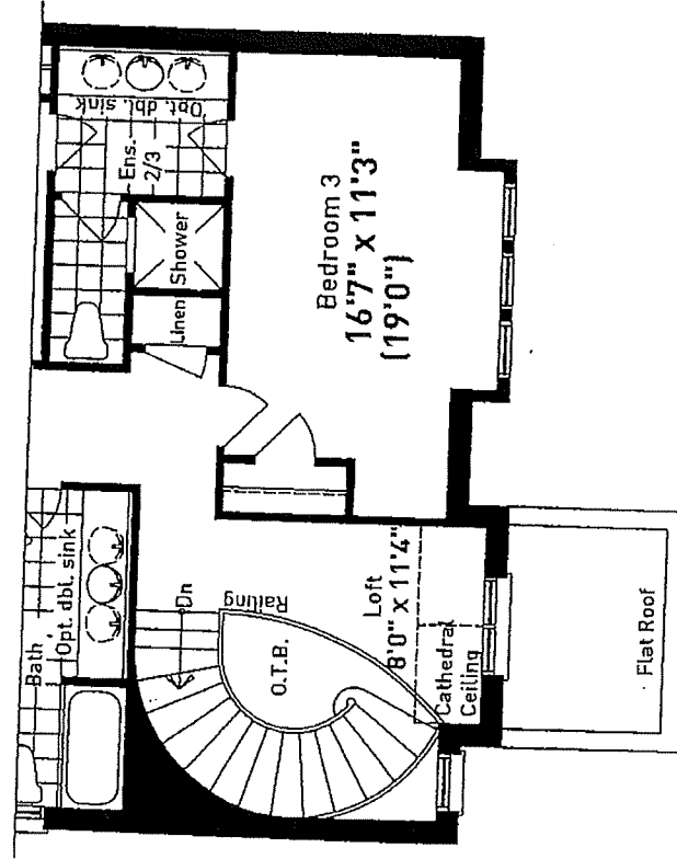
PARTIAL SECOND FLOOR PLAN ELEVATION C
