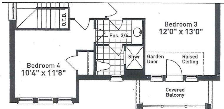
PARTIAL SECOND FLOOR PLAN ELEVATION C
