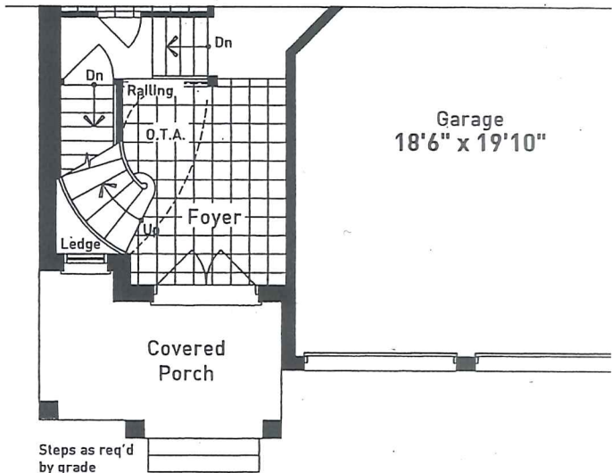
PARTIAL GROUND FLOOR PLAN ELEVATION B
