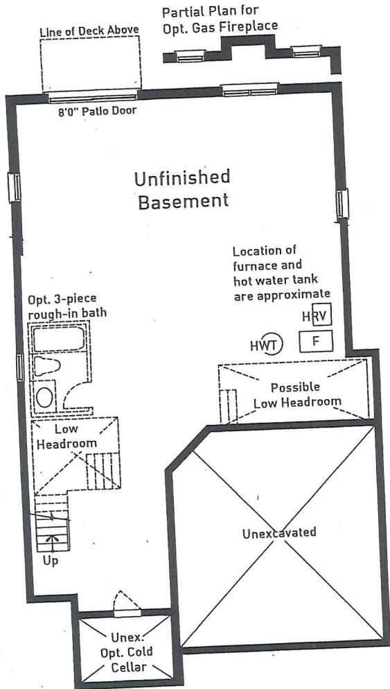
WALKOUT BASEMENT FLOOR PLAN ELEVATION A
