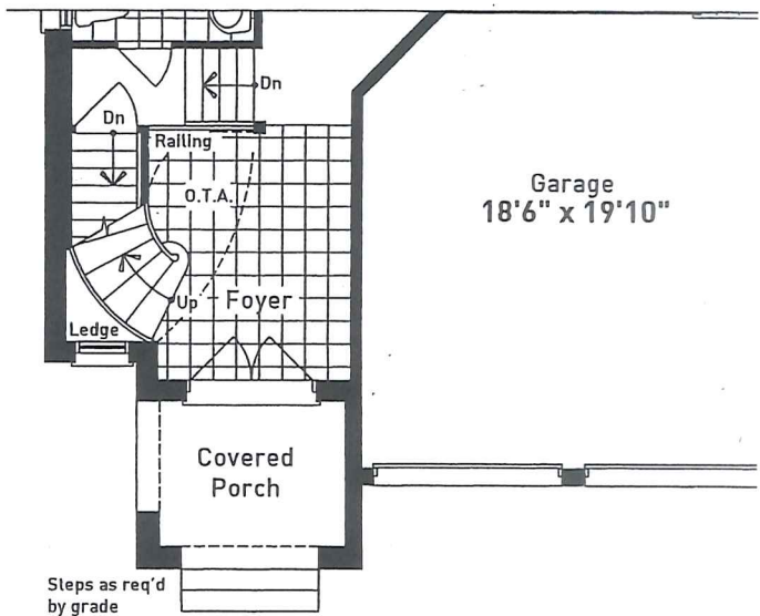
PARTIAL GROUND FLOOR PLAN ELEVATION C
