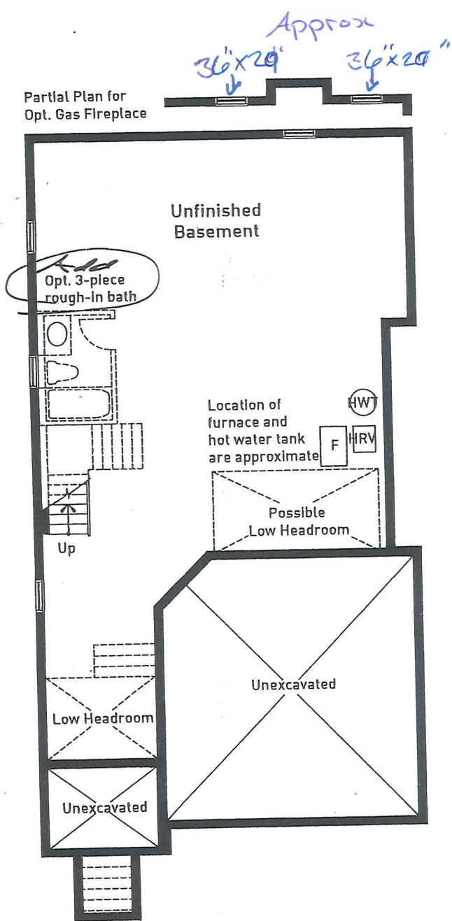
BASEMENT FLOOR PLAN ELEVATION B
