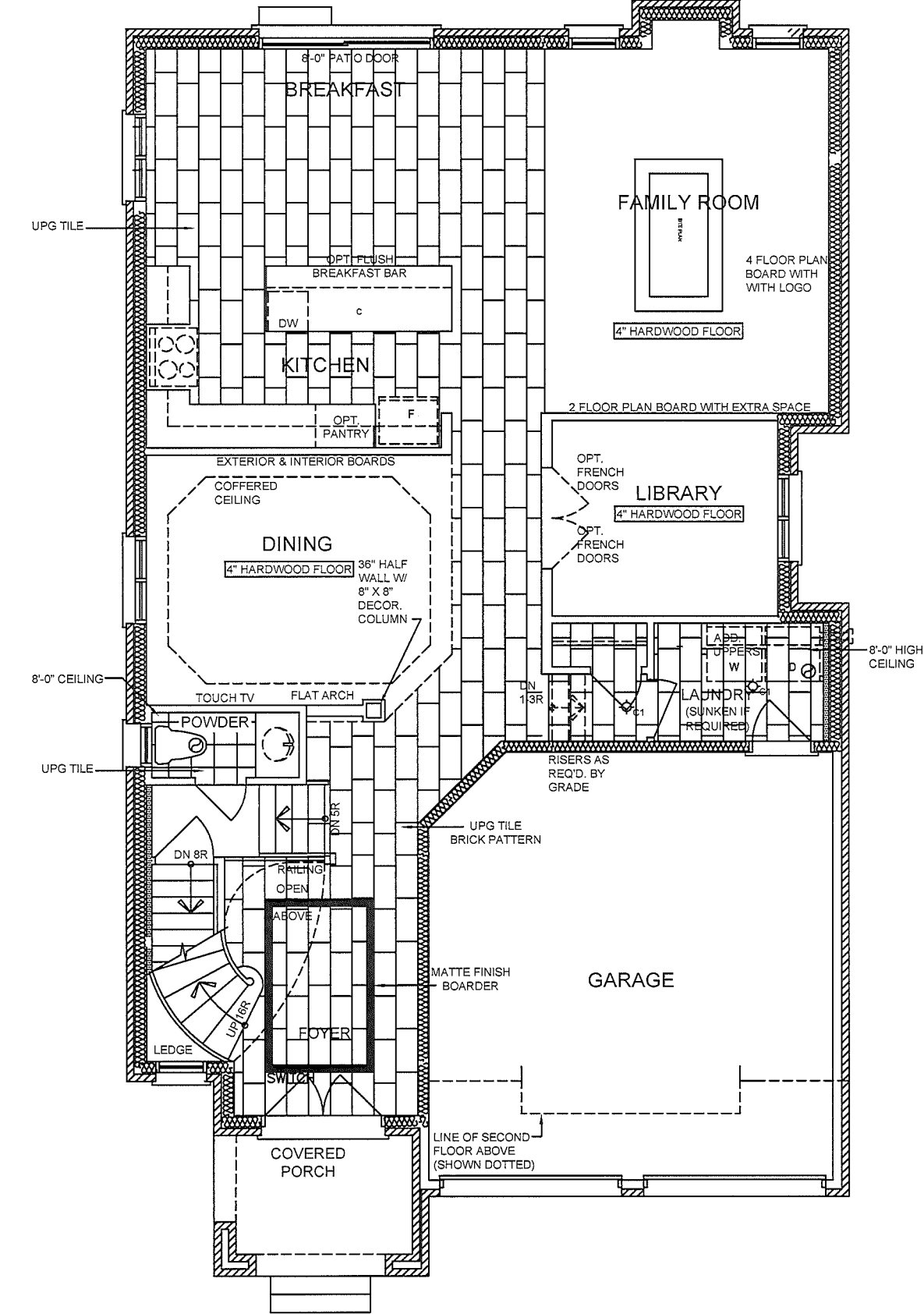
TILE LAYOUT
