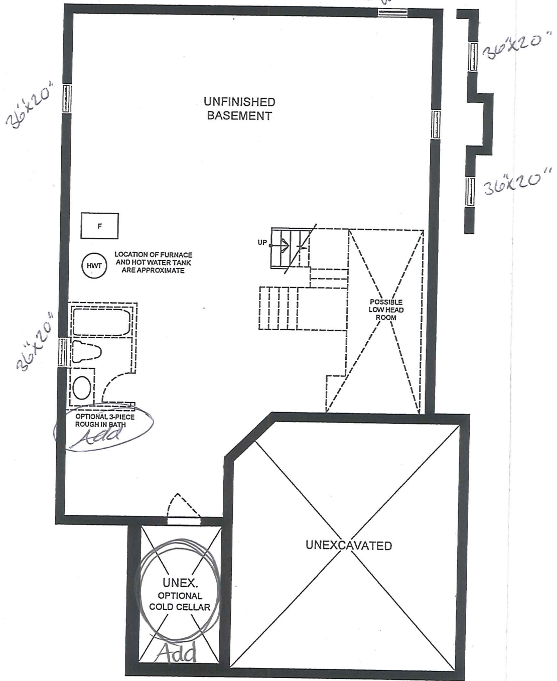
BASEMENT PLAN
