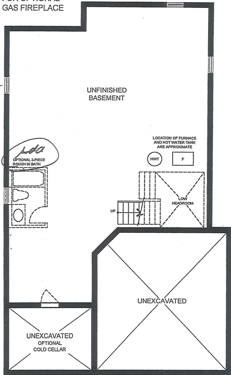
BASEMENT PLAN
