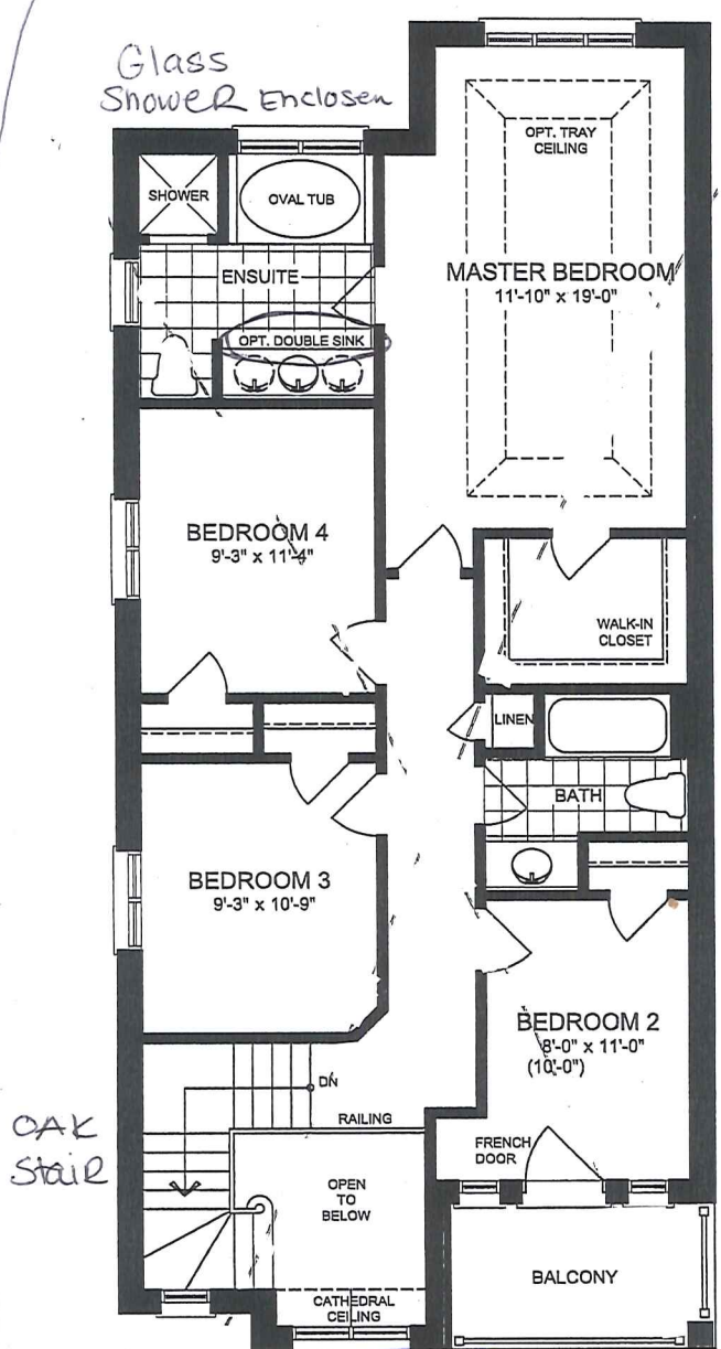
SECOND FLOOR PLAN OPTIONAL 4 BEDROOM ELEVATION 'B'
