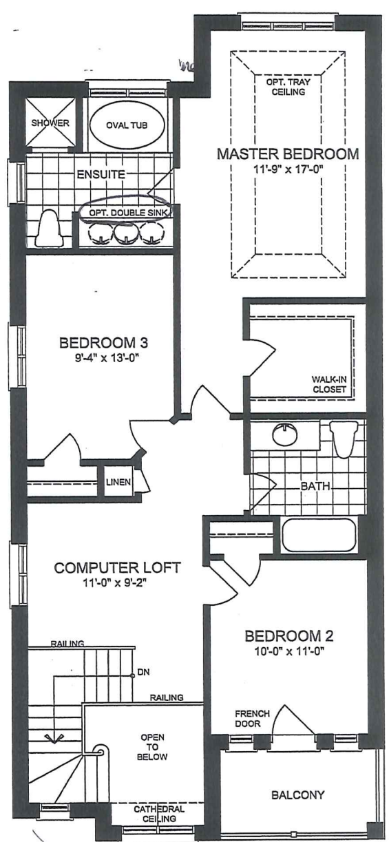
SECOND FLOOR PLAN ELEVATION 'B'
