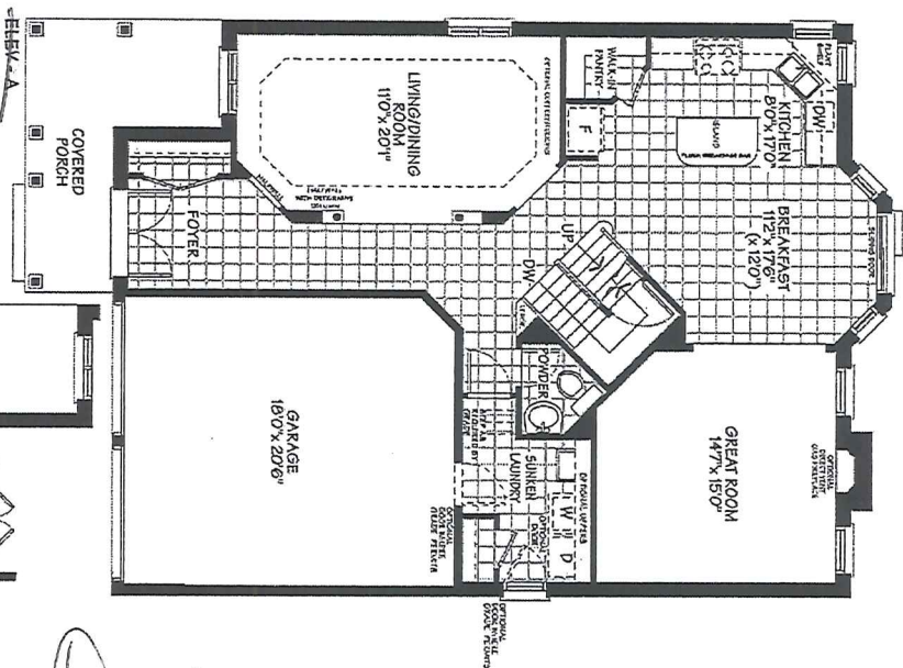
Elevation A - 2642 sq. ft.
