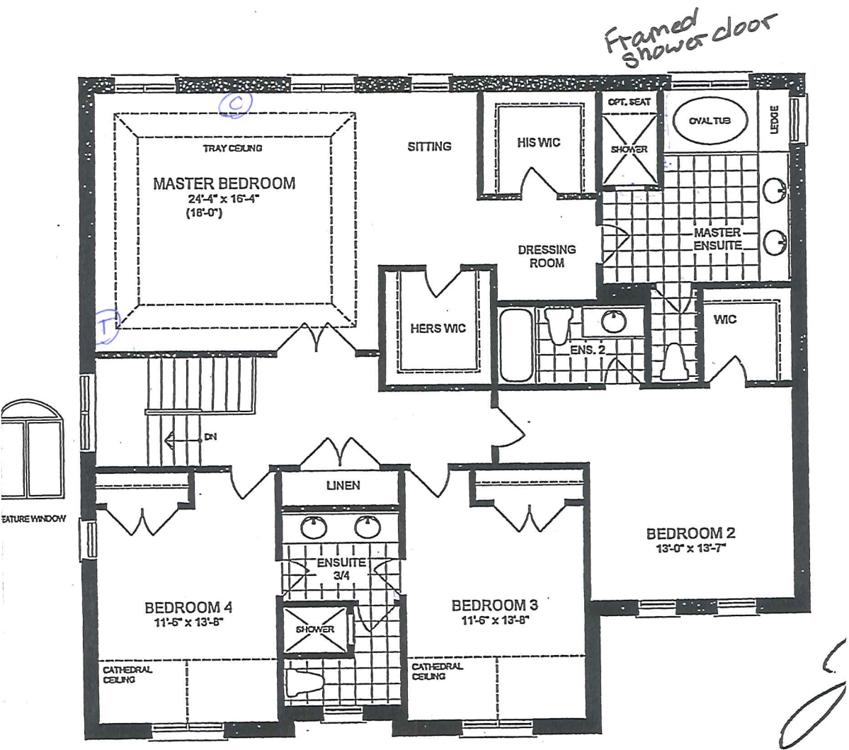
SECOND FLOOR PLAN ELEVATION C
