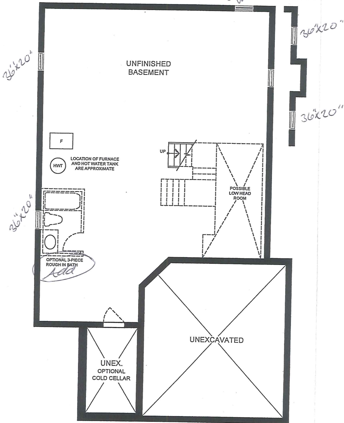
BASEMENT PLAN
