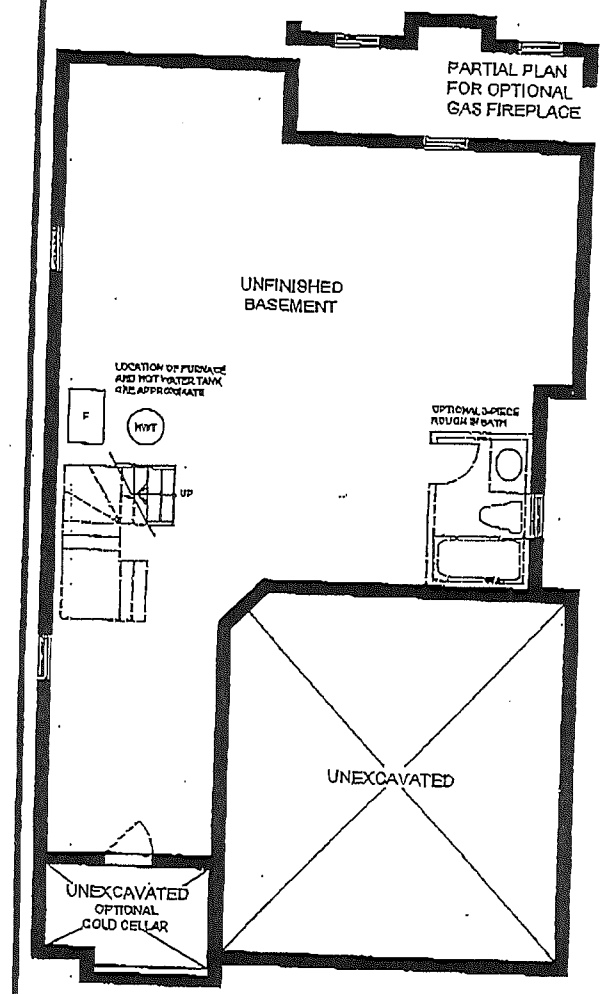
BASEMENT PLAN
