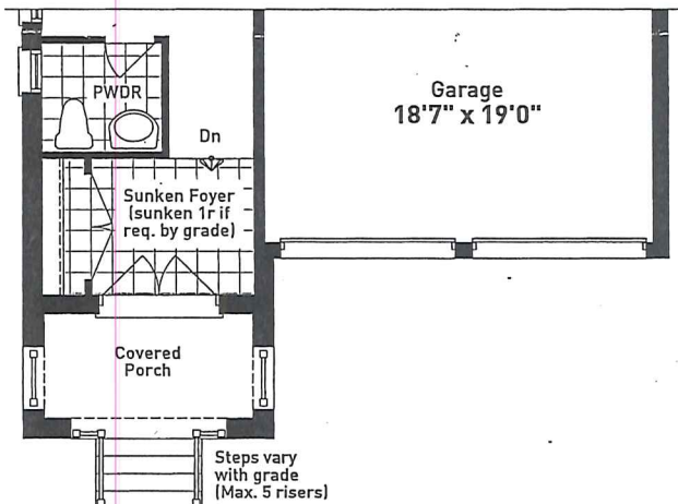
GROUND FLOOR PLAN ELEVATION C
