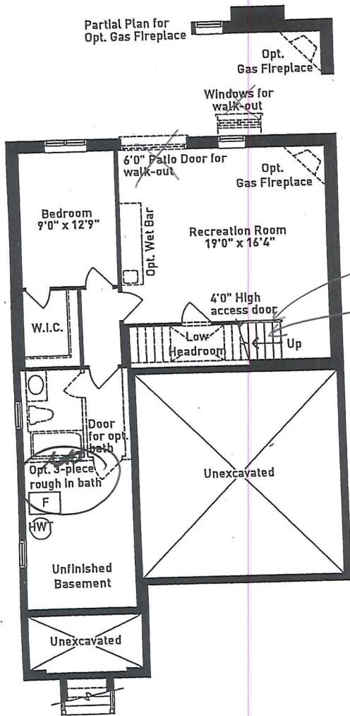
OPT. FINISHED BASEMENT PLAN W/ BEDROOM ELEVATION B
