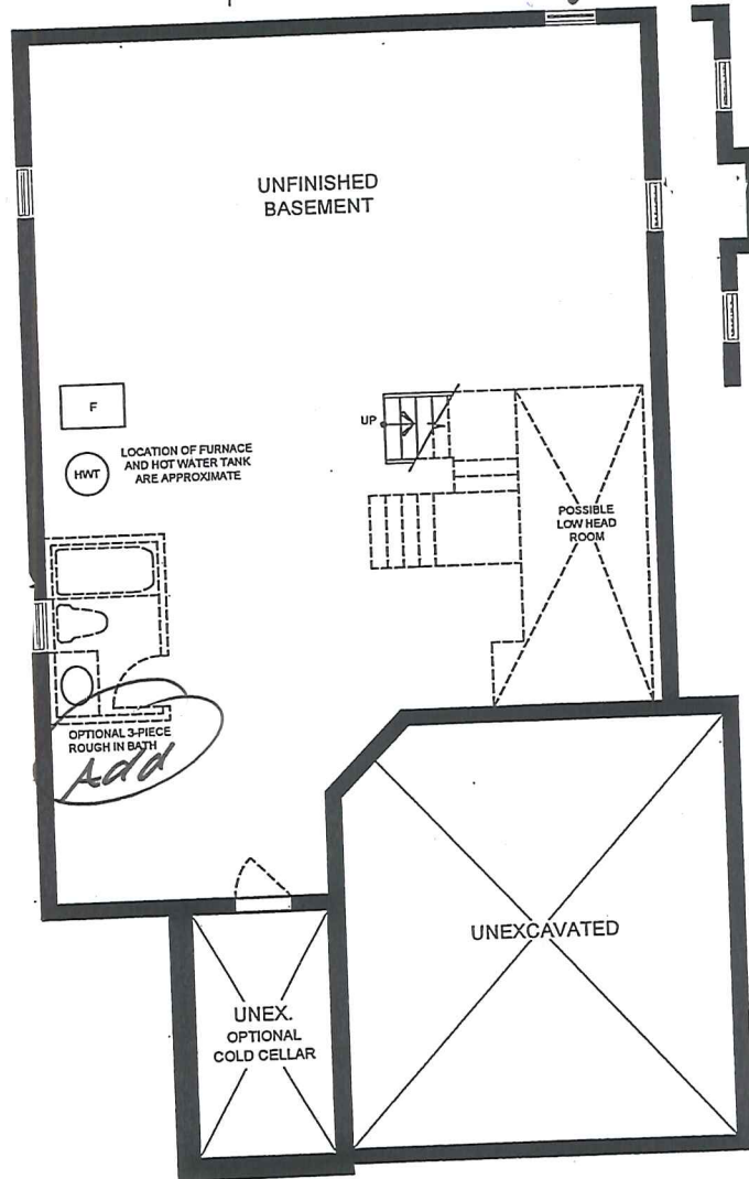
BASEMENT PLAN
