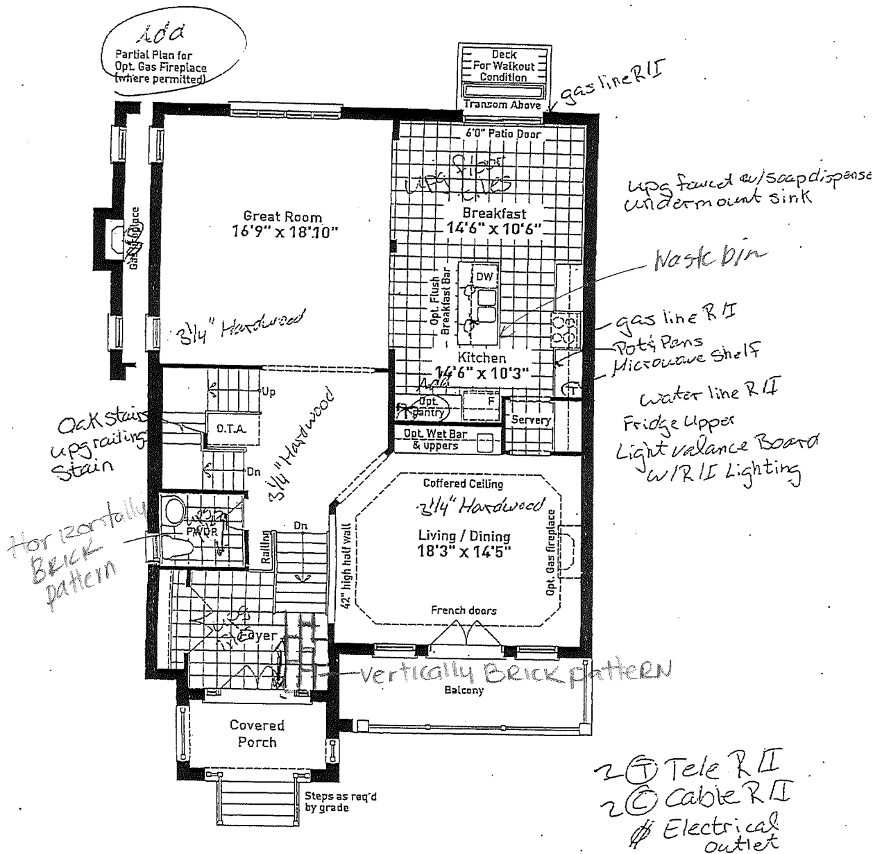
GROUND FLOOR PLAN ELEVATION B
