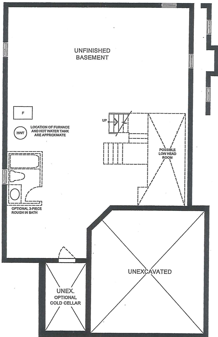
BASEMENT PLAN
