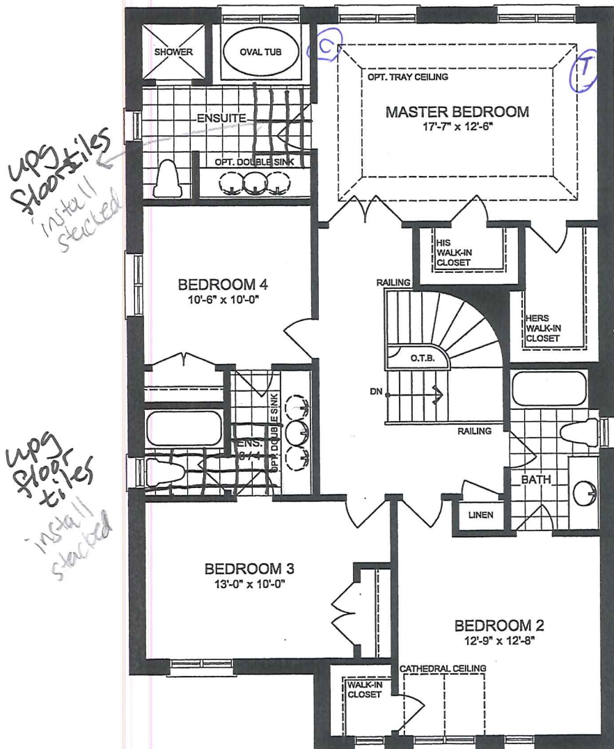
SECOND FLOOR PLAN ELEVATION 'B'
