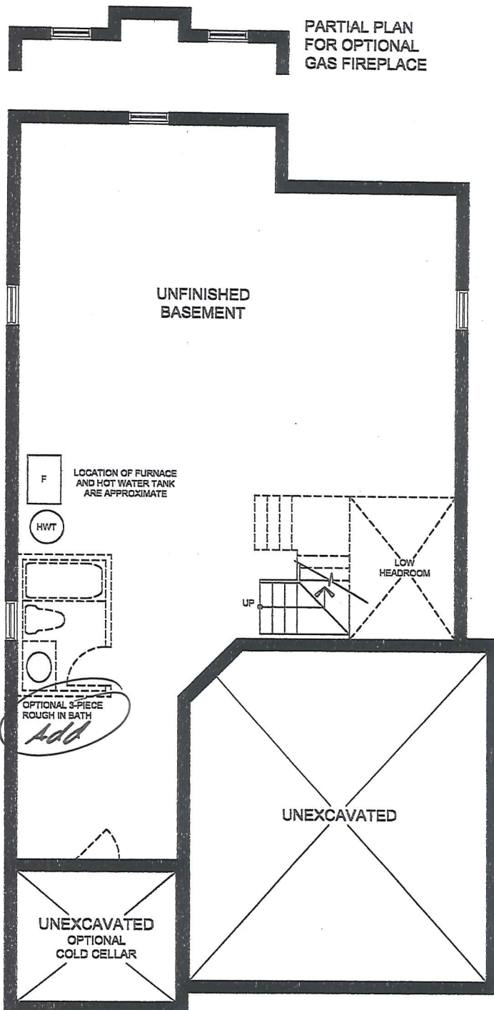
BASEMENT PLAN ELEVATION 'A' & 'B'
