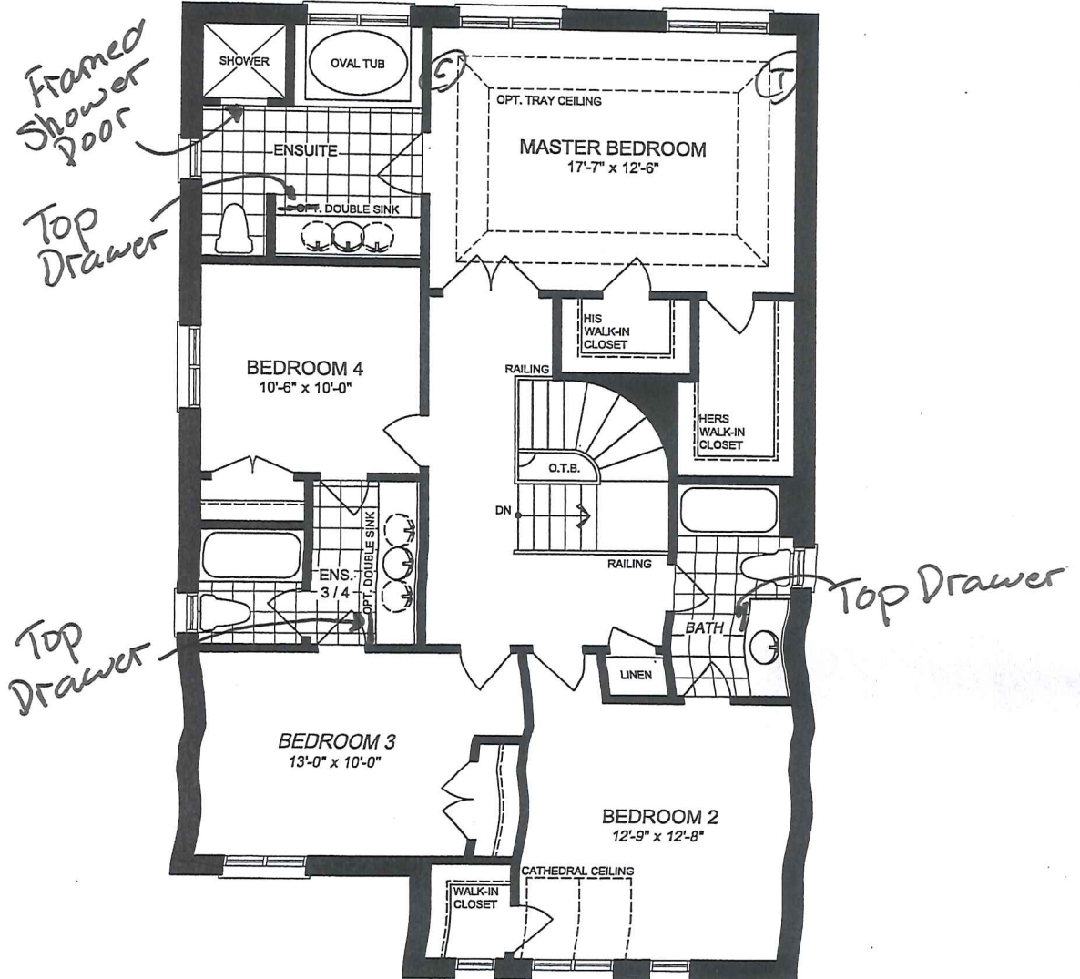
SECOND FLOOR PLAN ELEVATION 'B'
