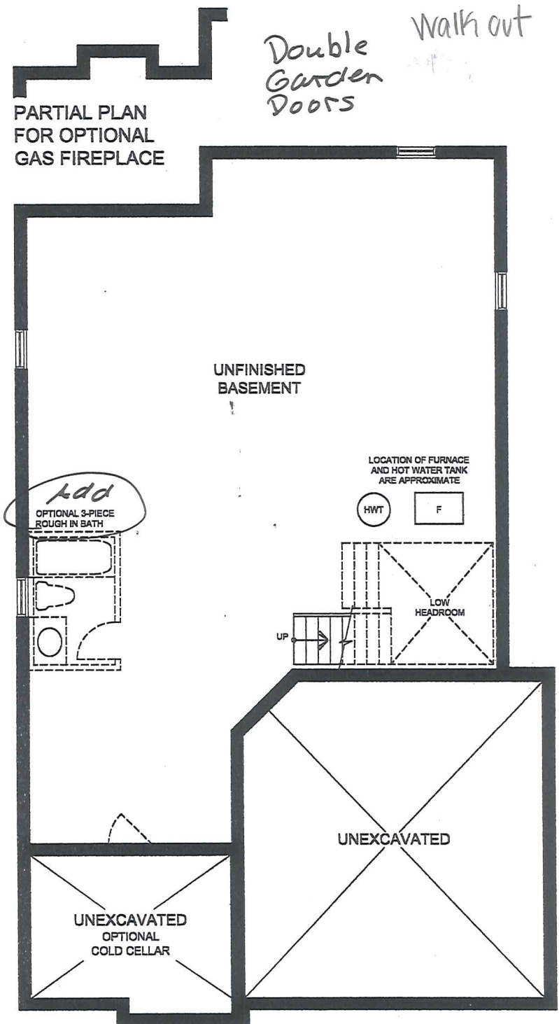
BASEMENT PLAN ELEVATION 'A'
