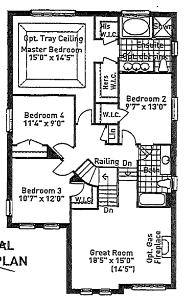
SECOND FLOOR PLAN ELEVATION C
