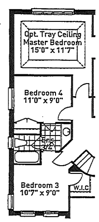
PARTIAL OPTIONAL SECOND FLOOR PLAN ELEVATION C
