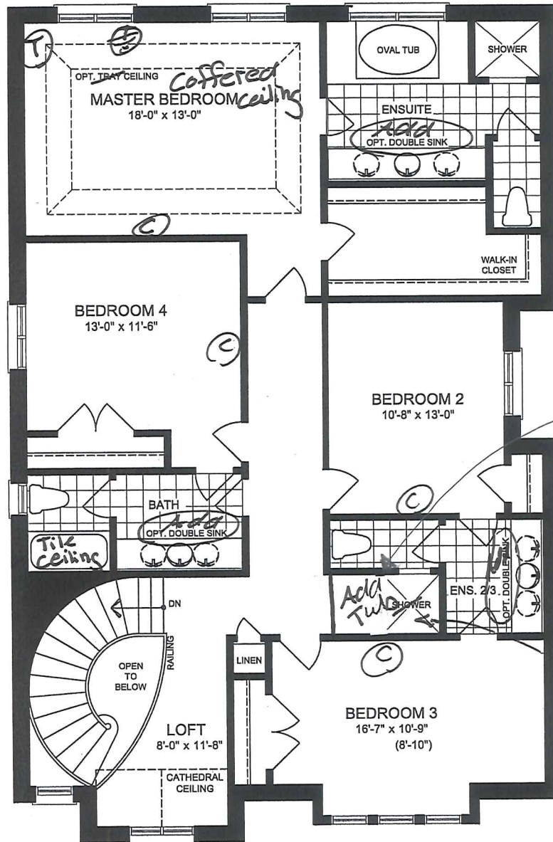
SECOND FLOOR PLAN ELEVATION 'C'
