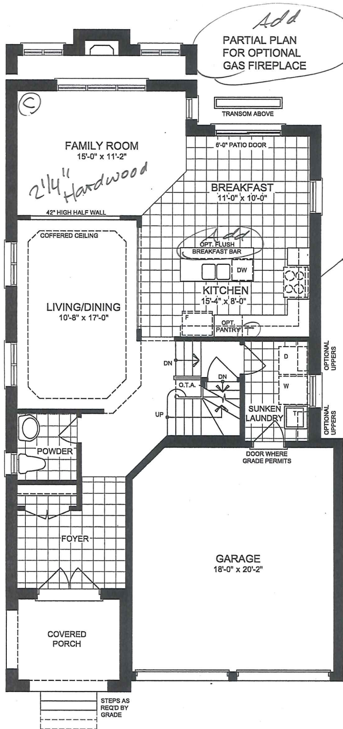
GROUND FLOOR PLAN ELEVATION 'C'
