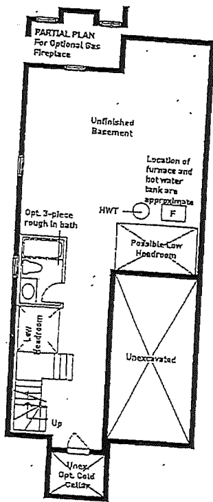
BASEMENT FLOOR PLAN ELEVATION A, B & C
