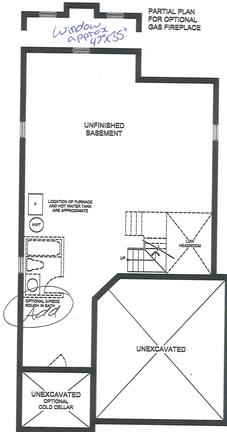
BASEMENT PLAN ELEVATION 'A' & 'B'
