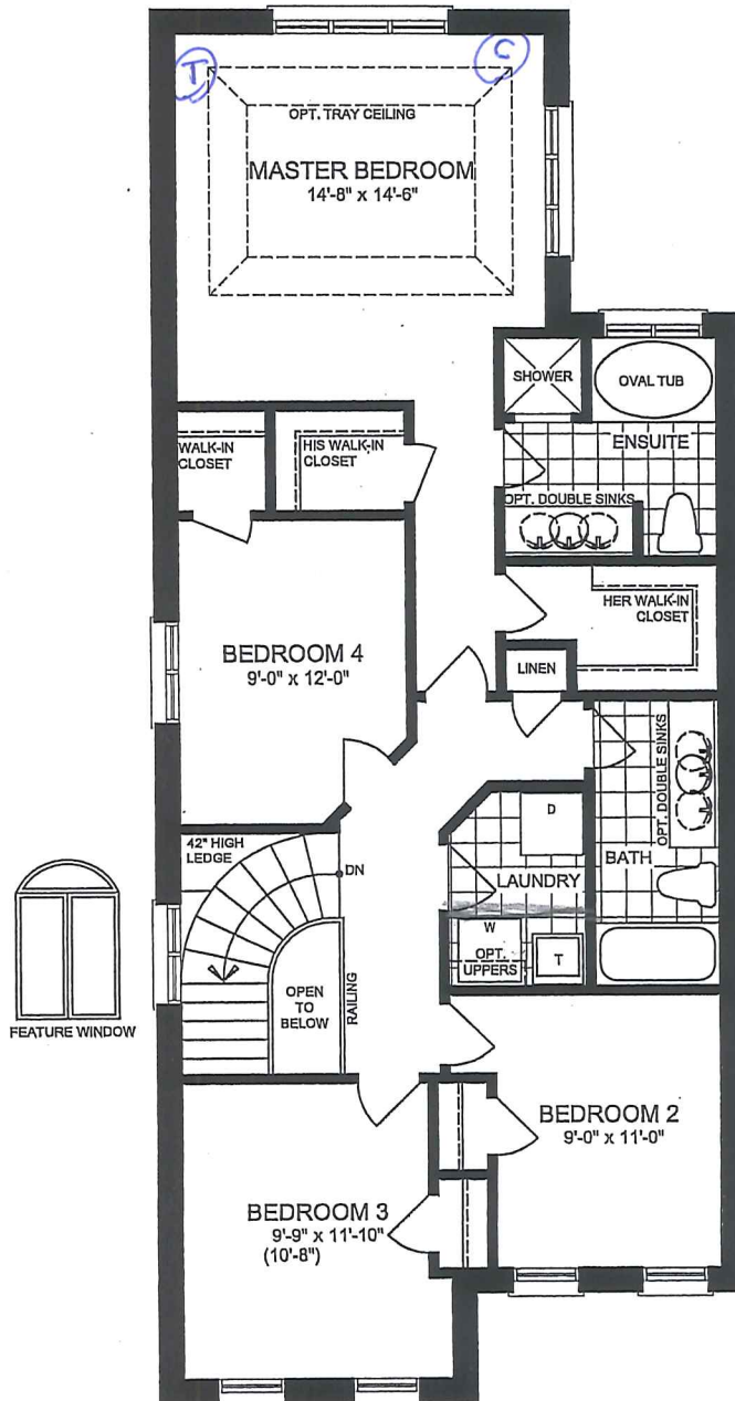
SECOND FLOOR PLAN ELEVATION 'B'
