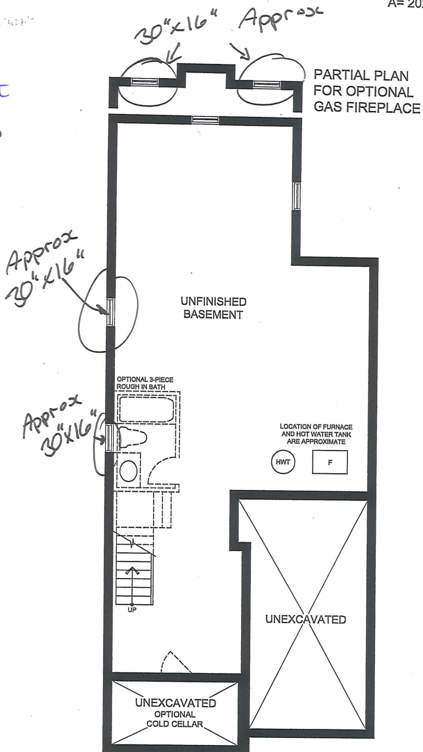
BASEMENT PLAN ELEVATION 'B'
