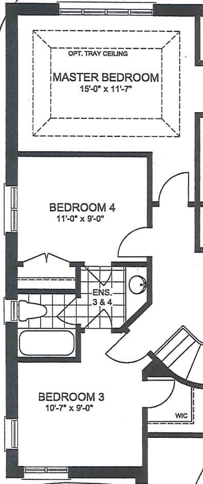
PARTIAL OPTIONAL SECOND FLOOR PLAN ELEVATION 'B'
