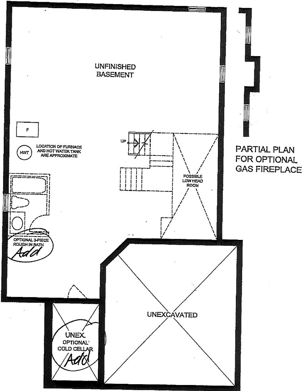
BASEMENT PLAN ELEVATION 'B'
