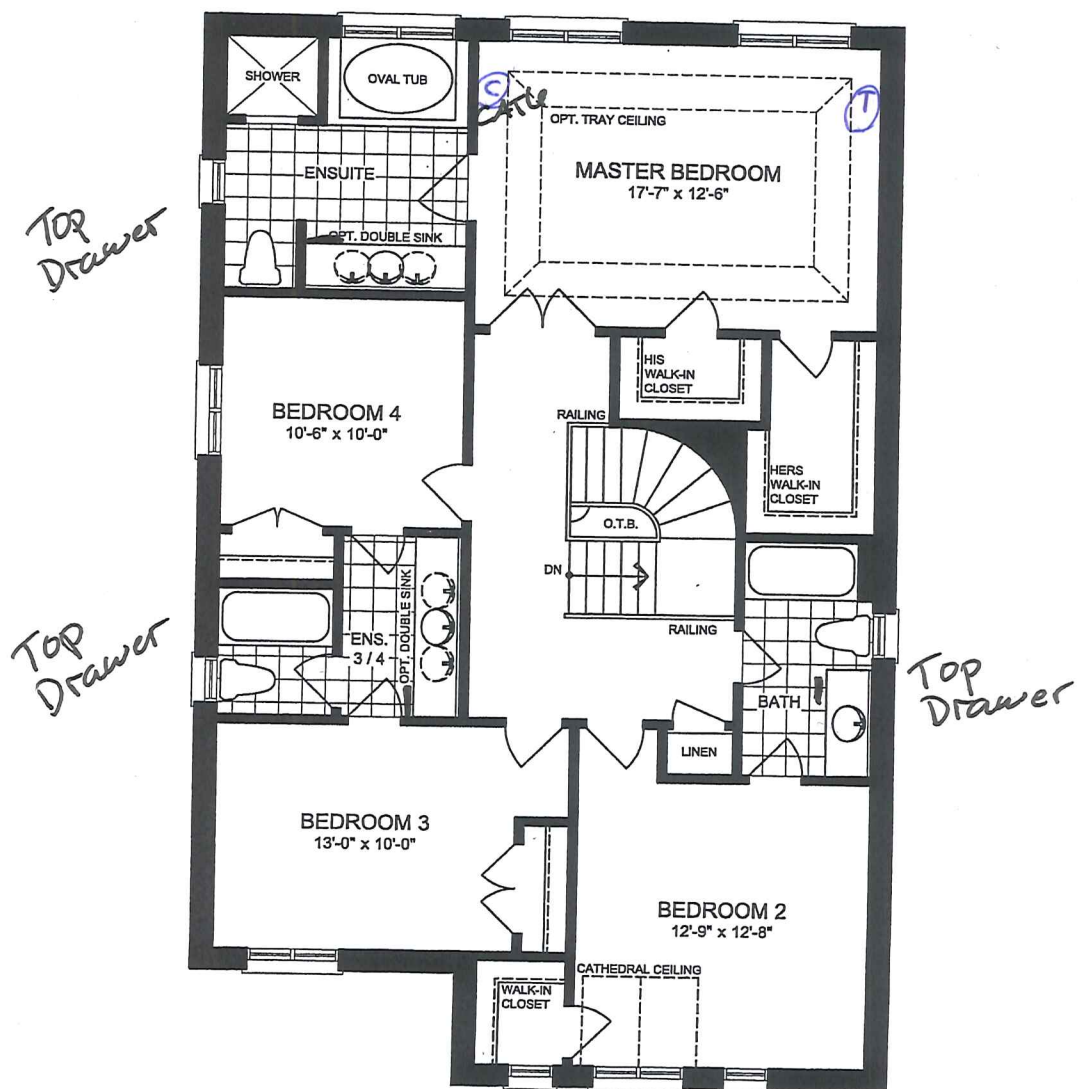
SECOND FLOOR PLAN ELEVATION 'B'
