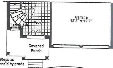
PARTIAL GROUND FLOOR PLAN ELEVATION B
