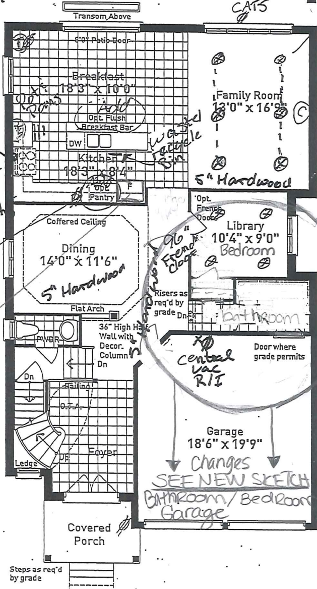
GROUND FLOOR PLAN ELEVATION A Garden Doors
