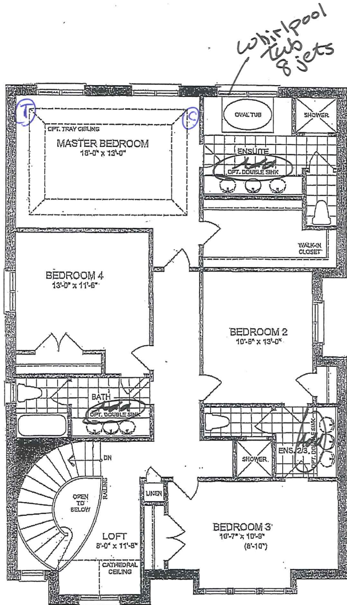
SECOND FLOOR PLAN ELEVATION 'C'
