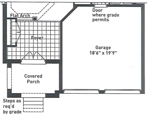
PARTIAL GROUND FLOOR PLAN ELEVATION B
