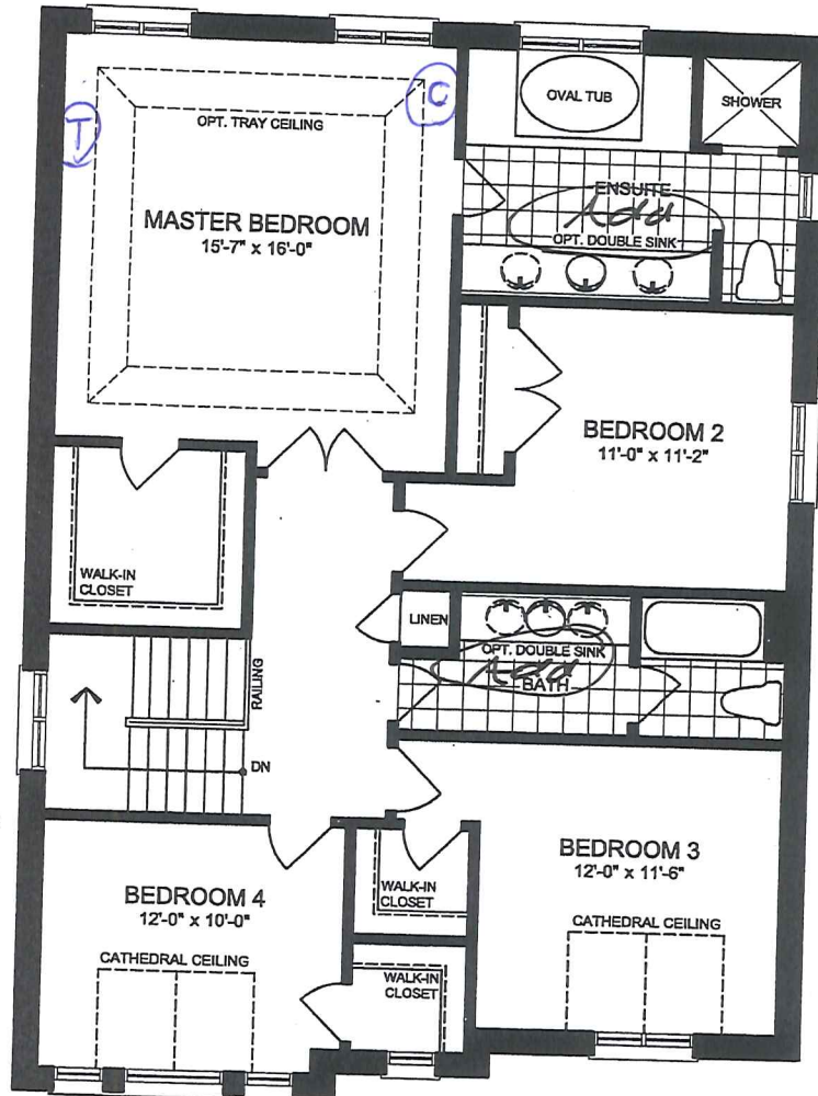
SECOND FLOOR PLAN ELEVATION 'C'
