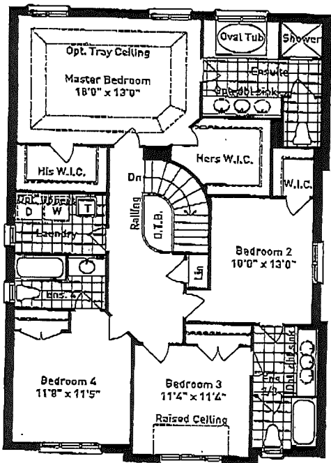
SECOND FLOOR PLAN ELEVATION B
