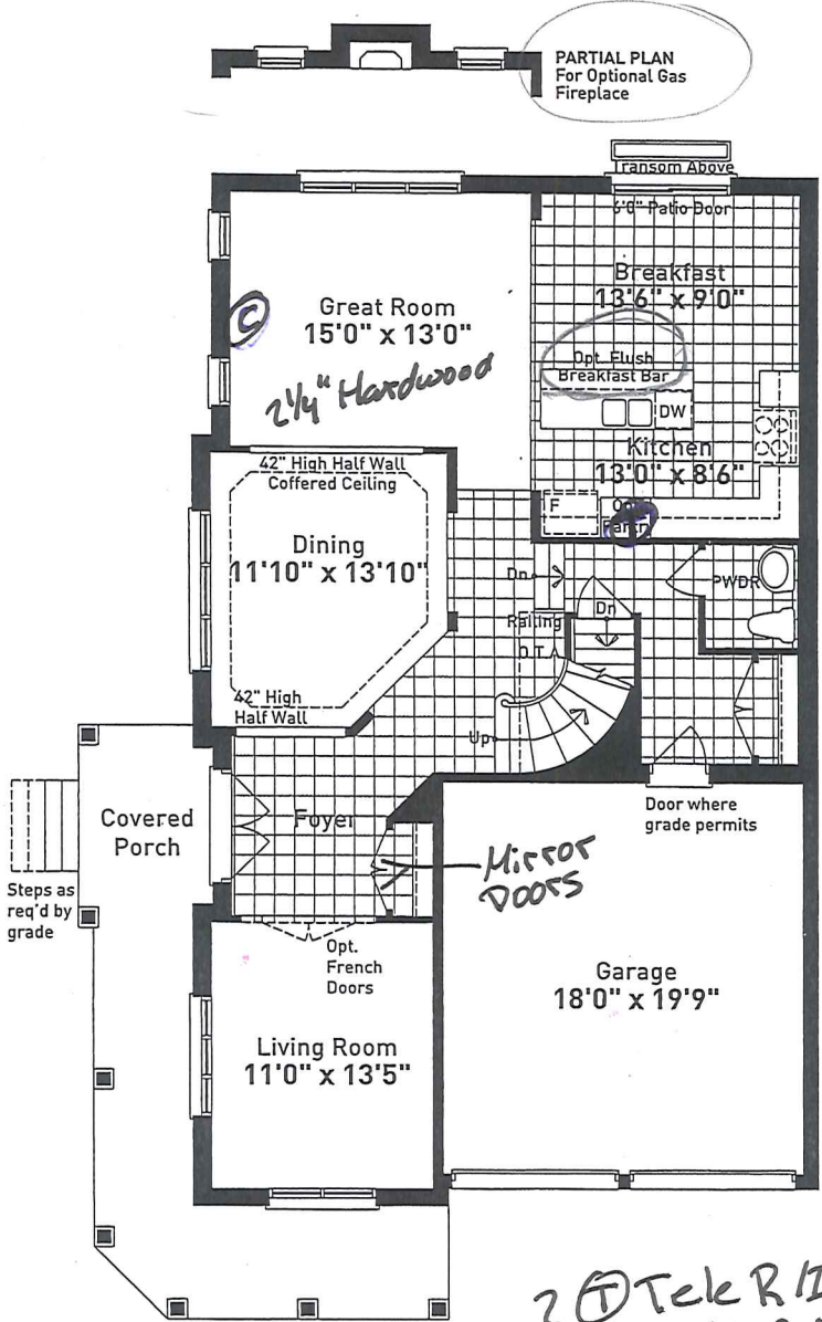
GROUND FLOOR PLAN ELEVATION A
