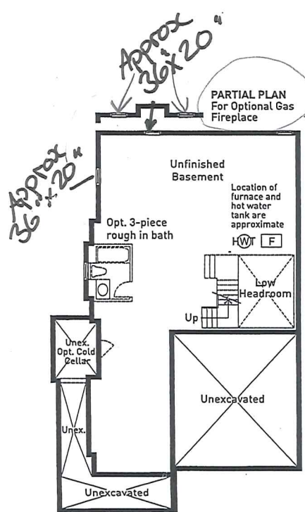
BASEMENT FLOOR PLAN ELEVATION B
