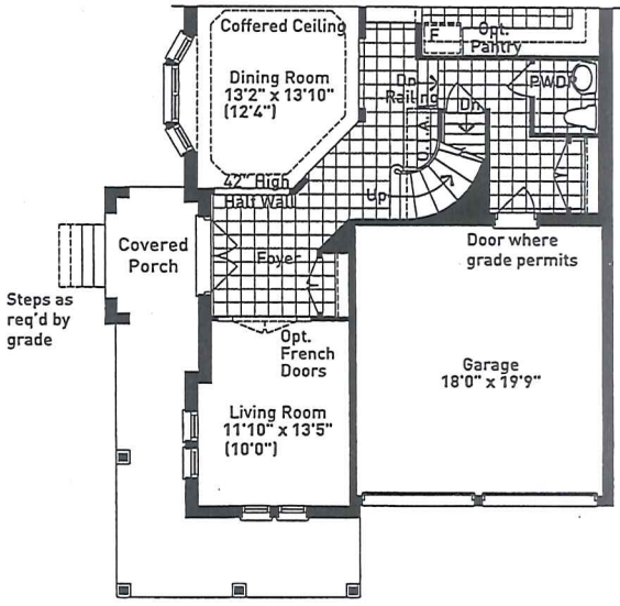
PARTIAL GROUND FLOOR PLAN ELEVATION C
