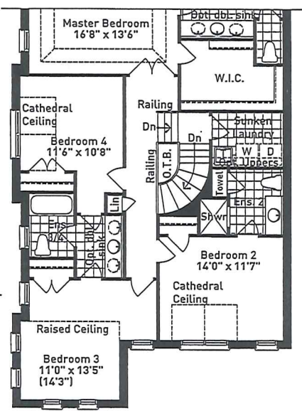
PARTIAL SECOND FLOOR PLAN ELEVATION C
