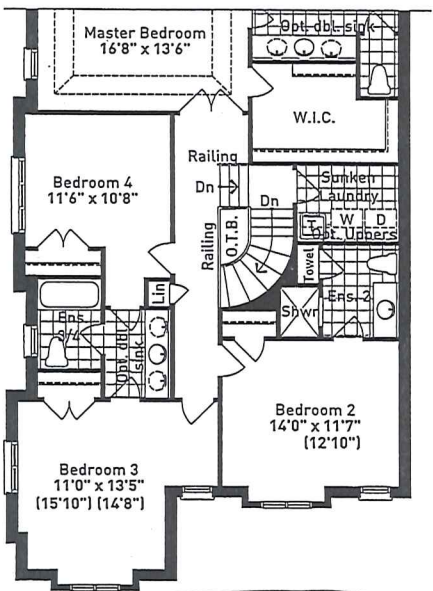
PARTIAL SECOND FLOOR PLAN ELEVATION B
