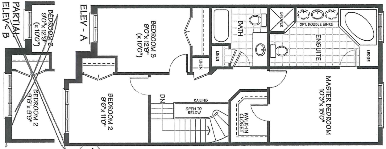
SECOND FLOOR
