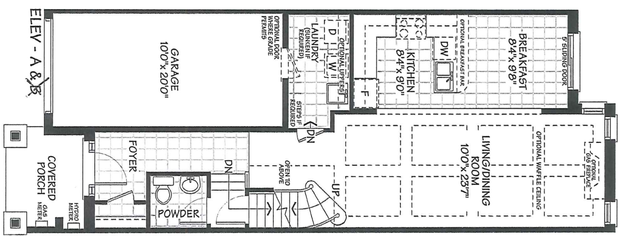
MAIN FLOOR
