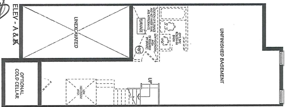
BASEMENT
