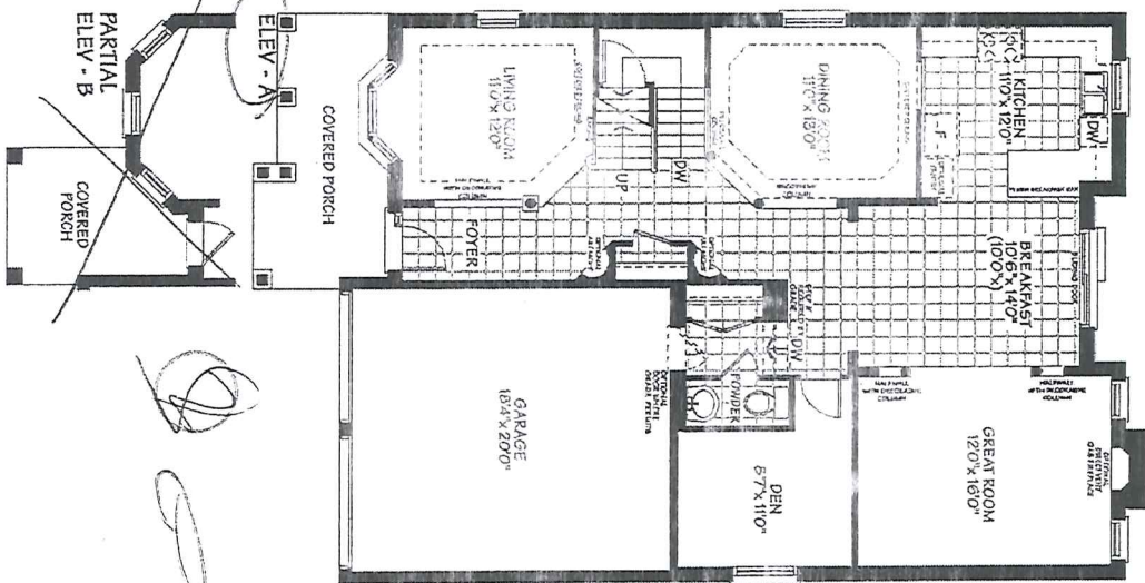
MAIN FLOOR
