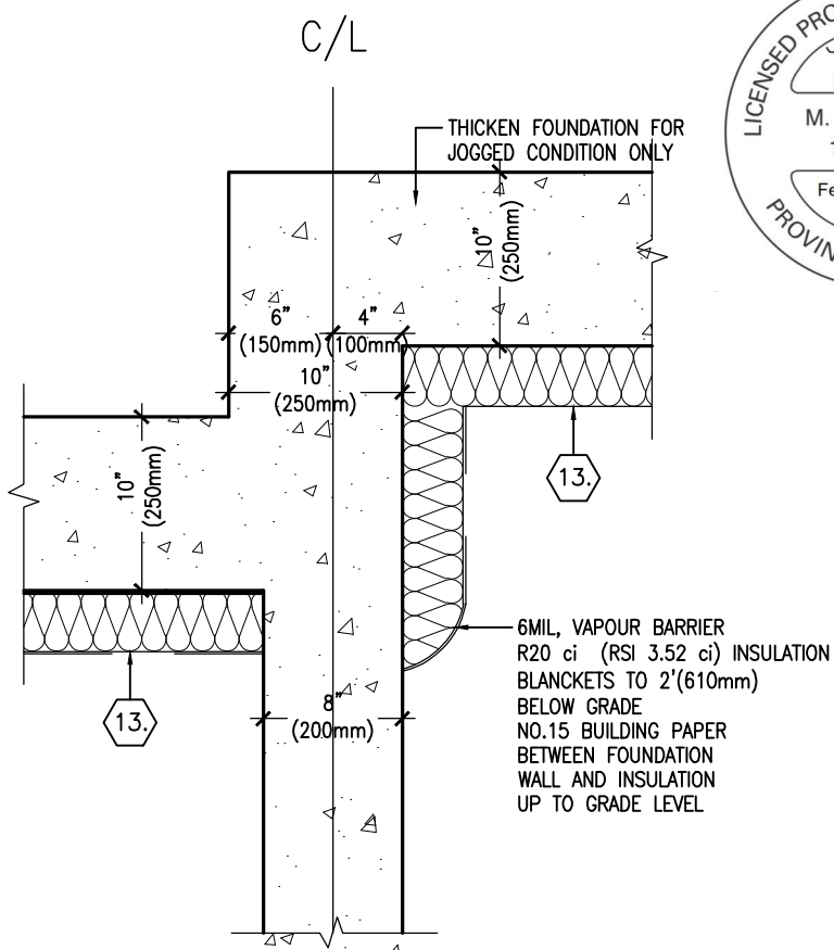
FOUNDATION WALL
