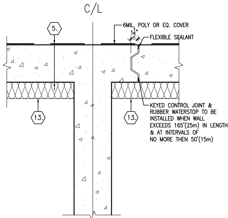
FOUNDATION WALL
