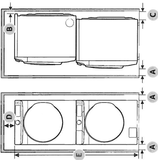
Stacked installation (Model: SKK-8K)
